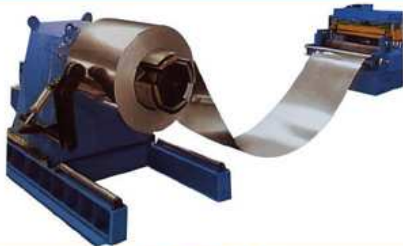
D-Coiler Machine
